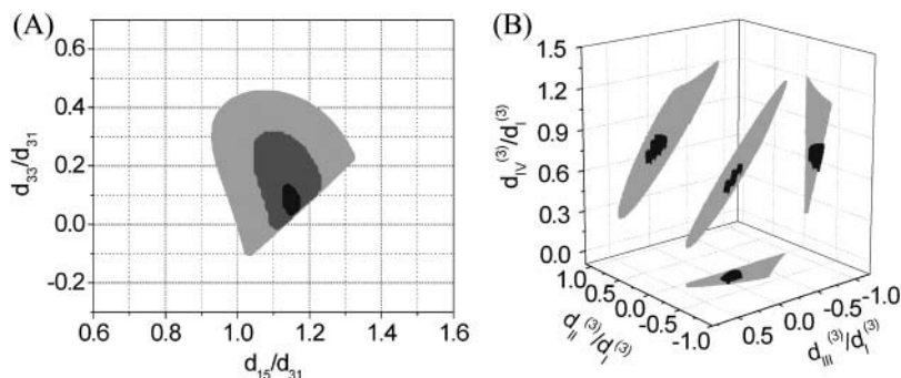
FIGURE 6 (A) The solution set for d_{15}/d_{31} and d_{33}/d_{31} depending on the allowed error range. The solid, shaded, and light shaded areas represent that fitting errors for SHG intensity are <0.43 , 0.45 , and 0.5 , respectively, whereas the errors for polarization orientation are all <0.48 . (B) The solution set for d_{II}^{(3)}/d_I^{(3)} , d_{III}^{(3)}/d_I^{(3)} , and d_{IV}^{(3)}/d_I^{(3)} , depending on the allowed error range. When the fitting error for THG intensity is <0.43 and for THG polarization orientation is <0.32 , all the possible solutions are plotted in the black area. When the constraint of THG intensity fitting error is relaxed to be <0.5 , the resulting expanded solution set is plotted in light shading.
